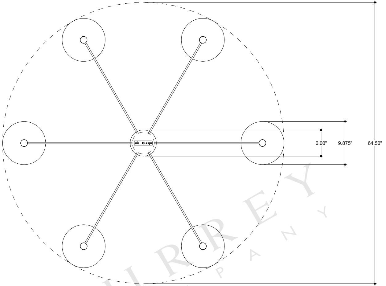
TOP VIEW
